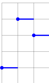
JSB 5: / (C,1) \ (F,1) \ (E,1)
