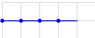
mms3: (C,1) (C,1) (C,1) (C,1)
