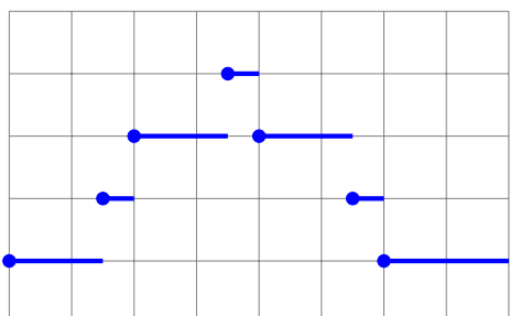
StaggerUpDown: (C,3/2) / (D,1/2) / (E,3/2) / (F,1/2) \setminus (E,3/2) \setminus (D,1/2) \setminus (C,2)
