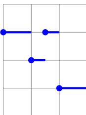
JSB 8: \ (C,1) \ (B,1/2) \ (C,1/2) (A,1)
