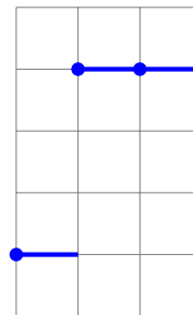
JSB 3: (C,1) \ (F,1) \ (F,1)
