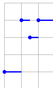
JSB 6: / (C,1) \ (F 1/2,1) \ (E,1/2) / (F,1)
